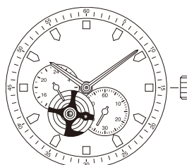
82S7 height 5.67mm / 21 jewels automatic and hand winding
