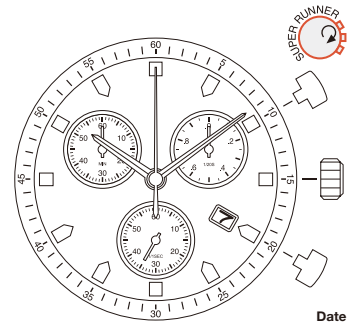
6S30 height 4.90mm chrono min / sec, 1/20 second 4 years battery life (SR927W)
